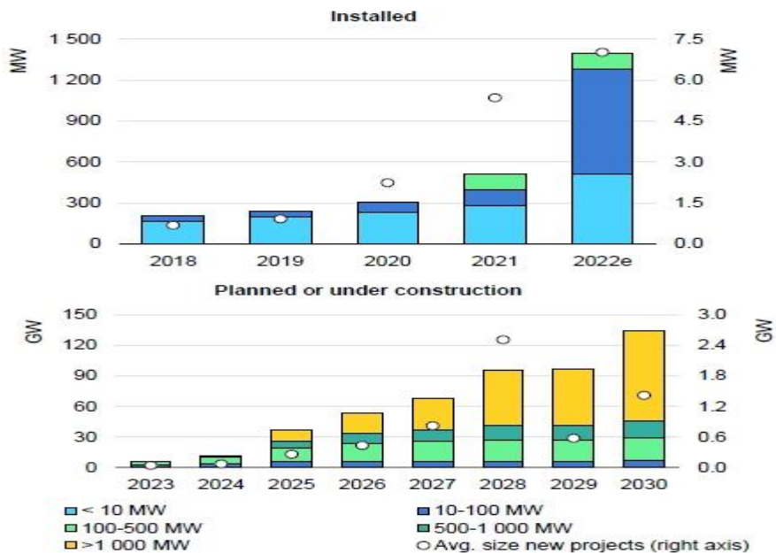
Global electrolyser capacity by size based on project pipeline, 2018-2030
